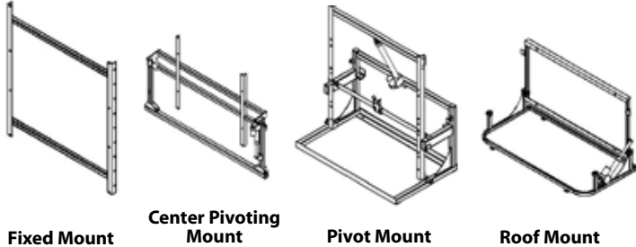
Examples of MOUNTS
