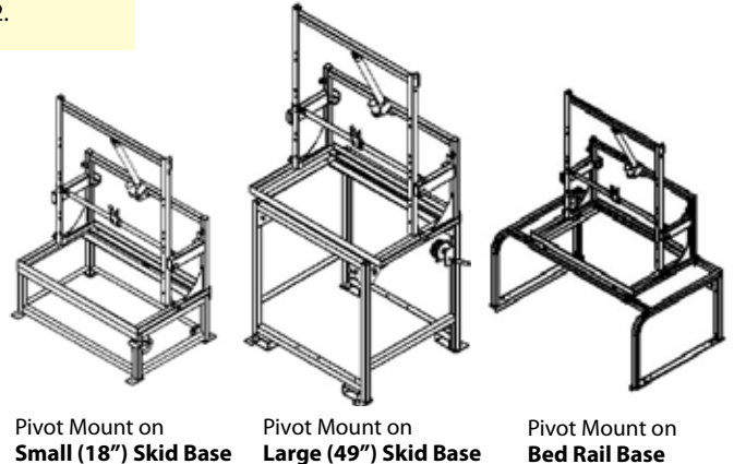
Examples of BASES
