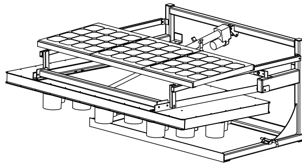
AT-PM 36"x72" B-Size Arrow Panel with Pivot Mount Shown w/ optional Solar Array
