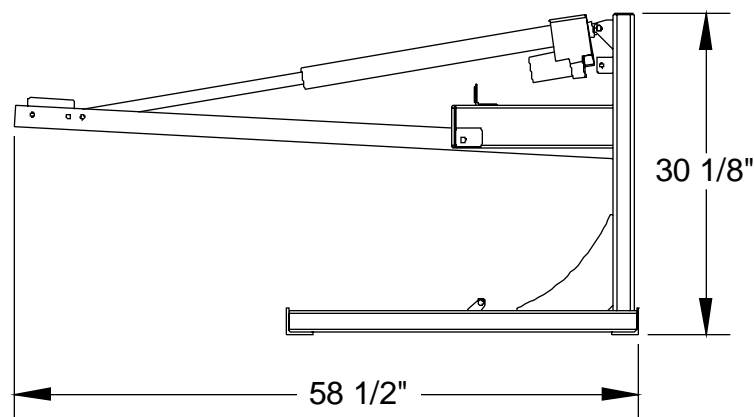
Side View Lowered
