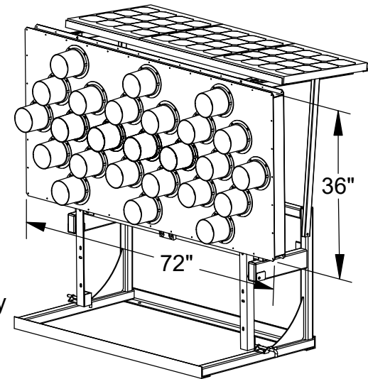
AT-PM 36"x72" B-Size Arrow Panel with Pivot Mount Shown w/ optional Solar Array
