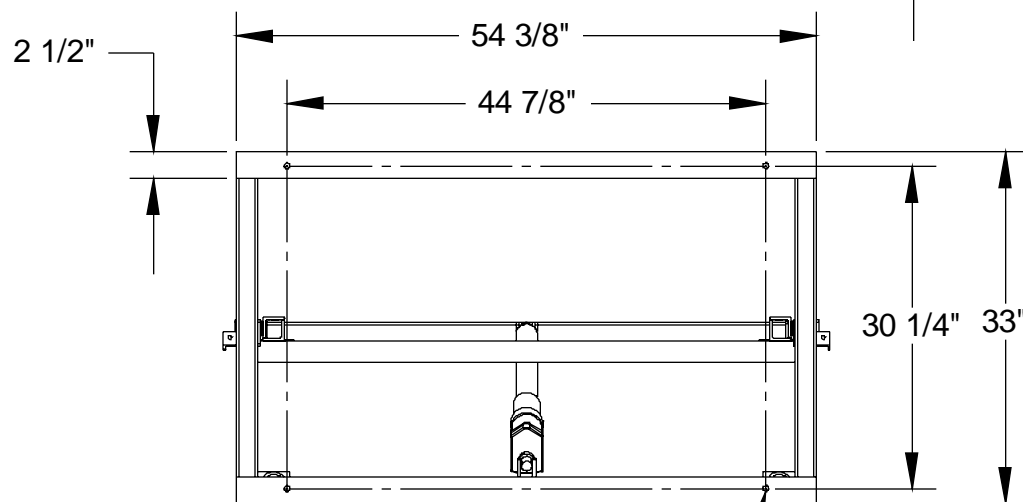
Front View
