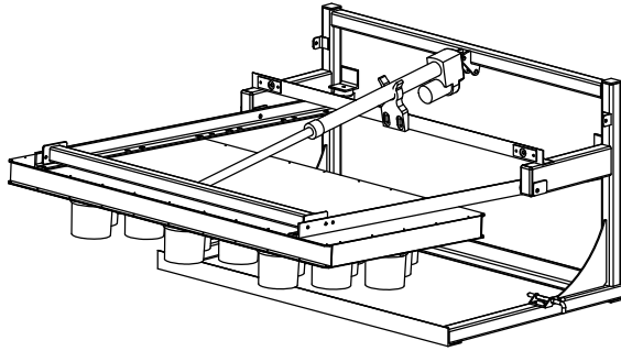
AT-PM 30"x60" B-Size Arrow Panel with Pivot Mount Weight: 220 lbs.
