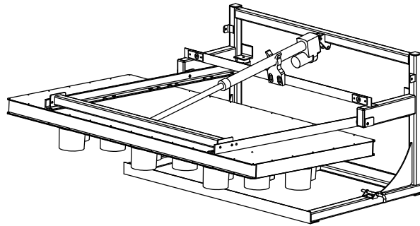
AT-PM 36"x72" B-Size Arrow Panel with Pivot Mount Weight: 235 lbs.
