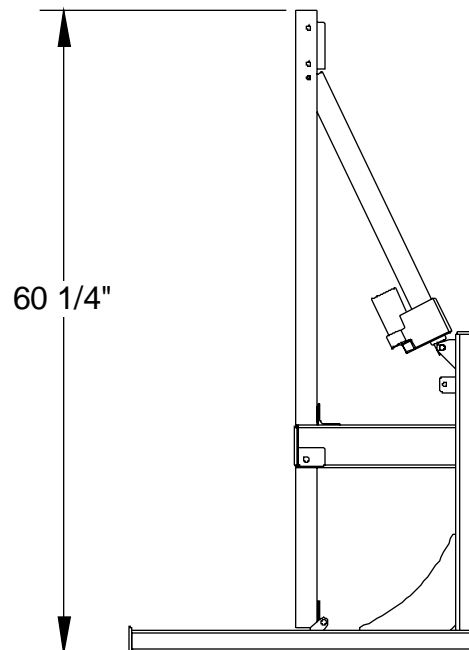
Side View Raised
