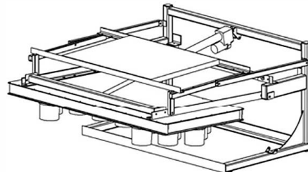
Pivot Mount AB Type-B
