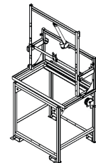
Pivot Mount on 37" or 49" Skid Base
