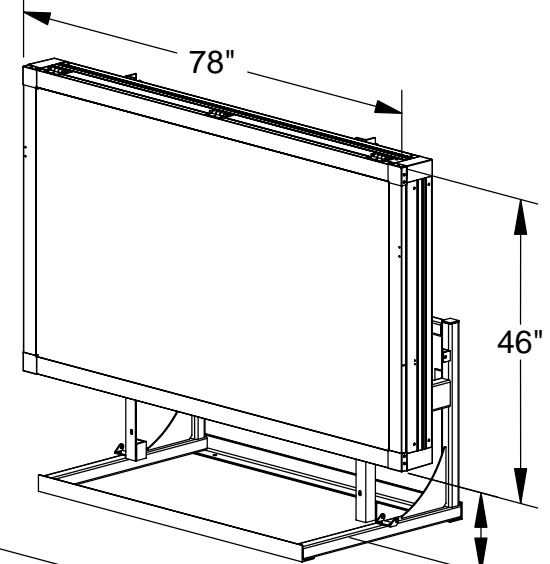
MT3-MP Silent Messenger III with Pivot Mount Weight: 305 lbs.
