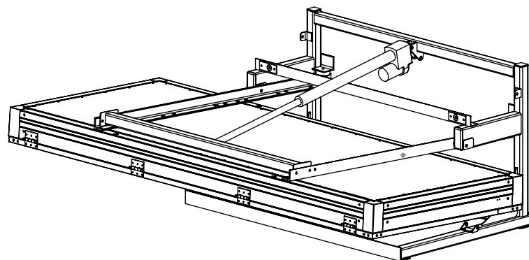
MT3-2-MP Silent Messenger III 2-Line Display with Pivot Mount Weight: 285 lbs.
