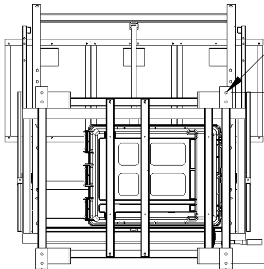
Front View Lowered
