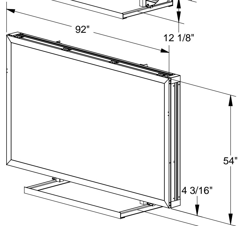
MT2-MP Silent Messenger II with Pivot Mount Weight: 350 lbs.
