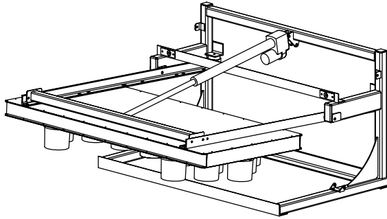
ATB-MP B-Size Arrow Panel with Pivot Mount Weight: 220 lbs.
