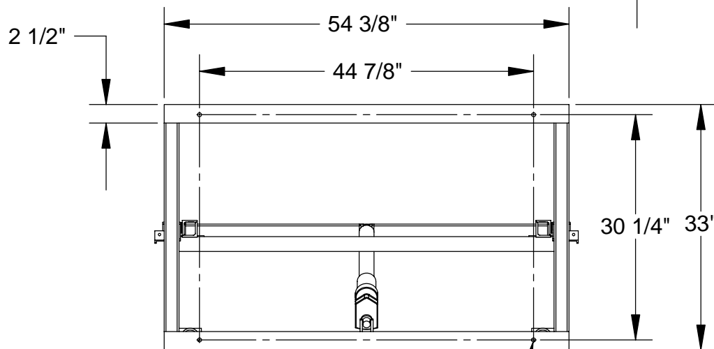
Front View
