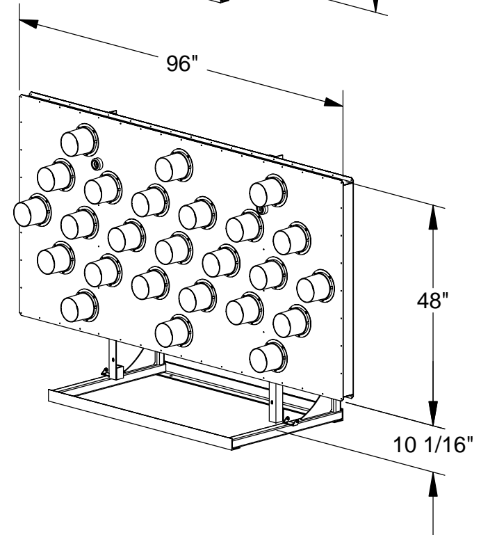
ATC-MP C-Size Arrow Panel with Pivot Mount Weight: 260 lbs.
