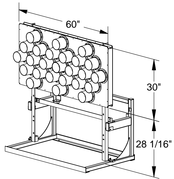
ATB-MP B-Size Arrow Panel with Pivot Mount Weight: 220 lbs.
