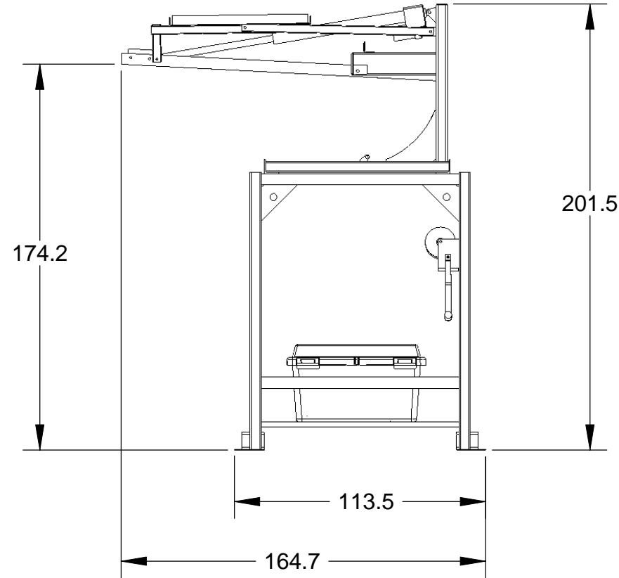
Side View Lowered
